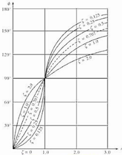
Fig. 4.3 Phase angle versus frequency ratio for different \zeta .
