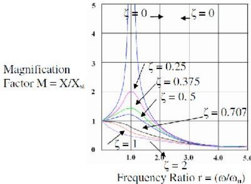
Magnification Factor vs Frequency Ratio for Different amounts of Damping
